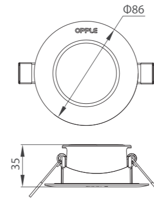
4.5W Downlight
